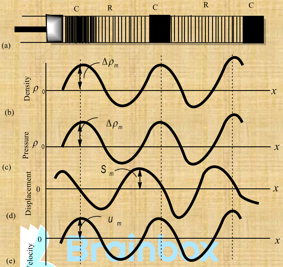
Fig. Sound Waves
