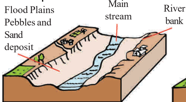
Fig 2.4 Flood Plains
