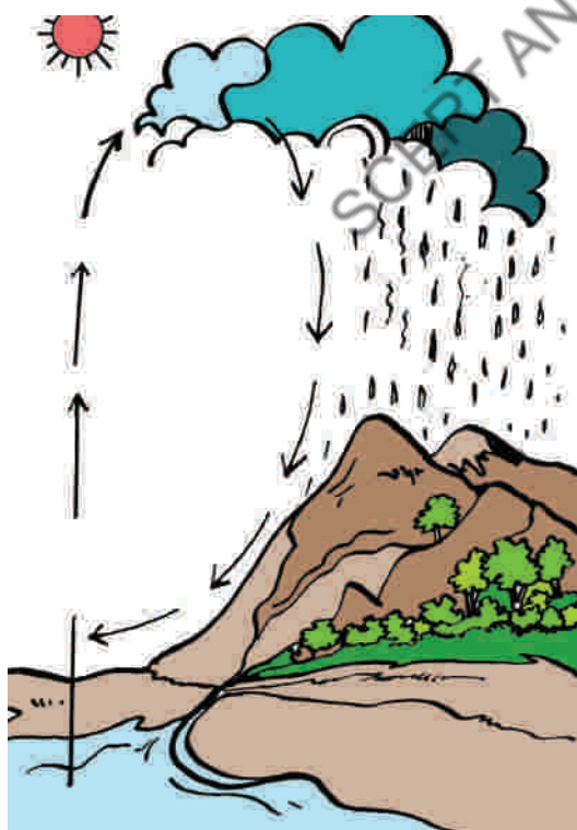
Fig 2.2 Water cycle
