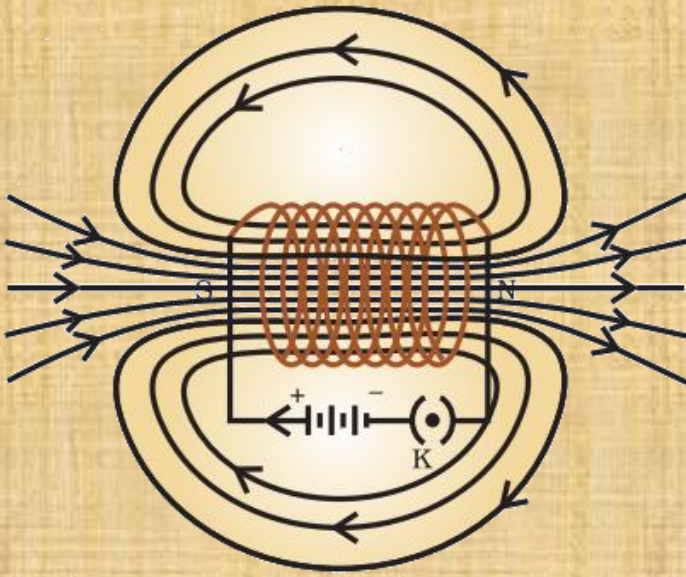
Fig. Field lines of the magnetic field through and around a current carrying solenoid
